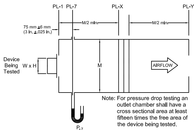
Figure 5.4- Test Device Setup with Outlet Chamber
