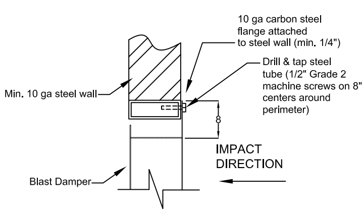
STEEL INSTALLATION
