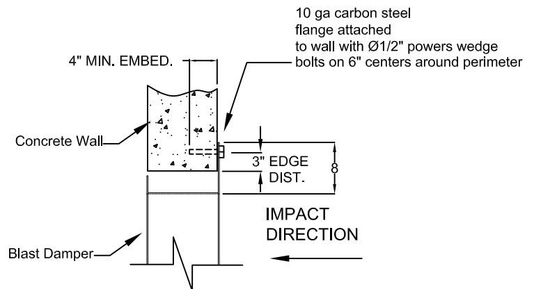
CONCRETE INSTALLATION
